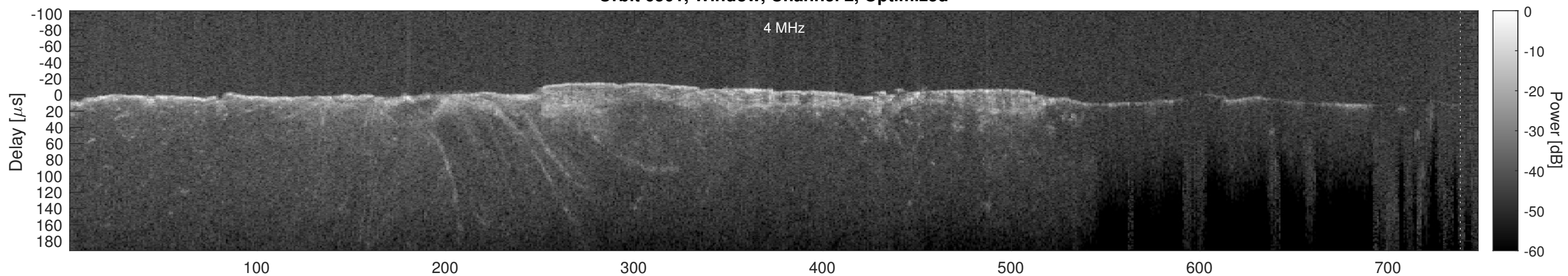
Orbit 6501, Cluttergram
