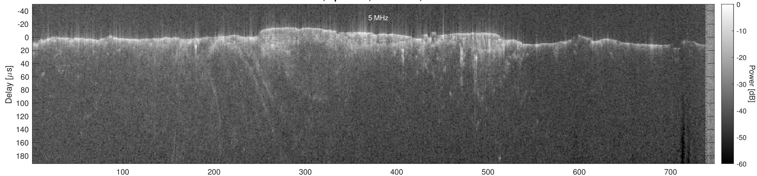
Orbit 6501, Optimized, No Window, Channel 2
