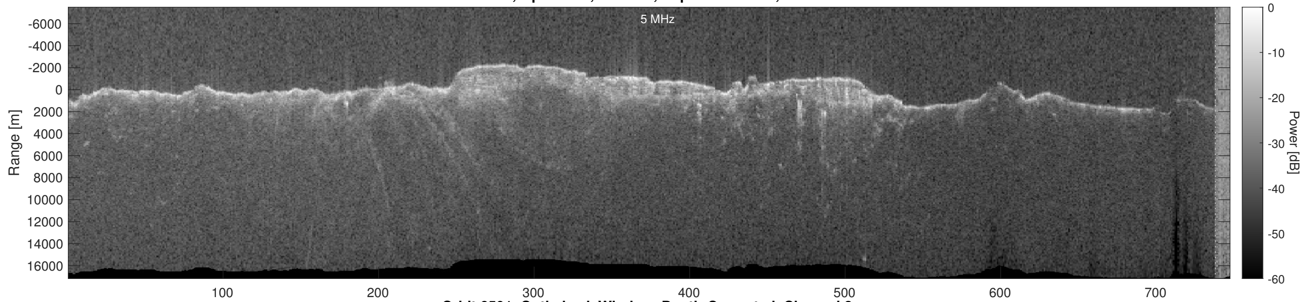
Orbit 6501, Optimized, Window, Depth-Corrected, Channel 2
