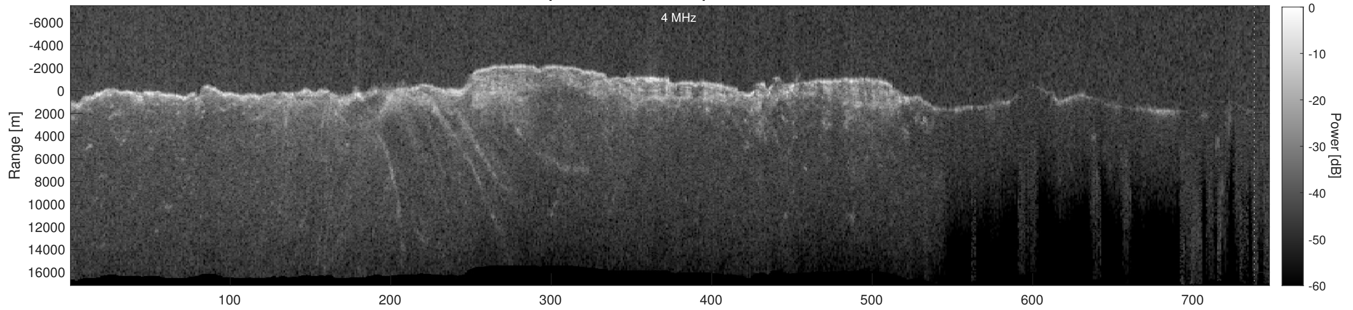
Orbit 6501, Depth-Corrected Cluttergram
