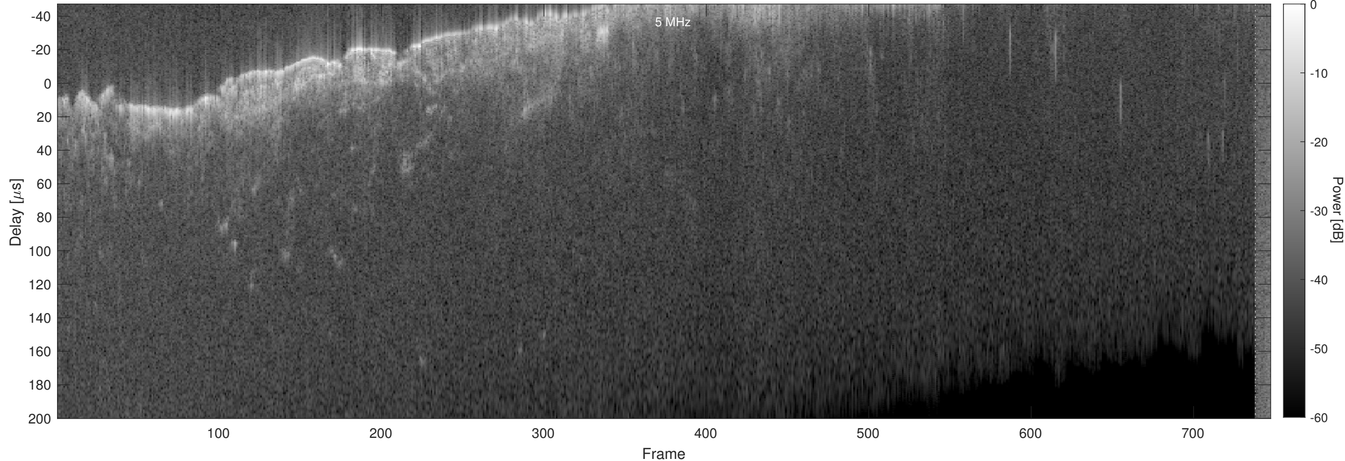
Orbit 6503, Chapman, No Window, Channel 2
