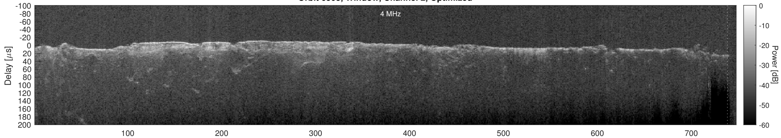
Orbit 6503, Cluttergram
