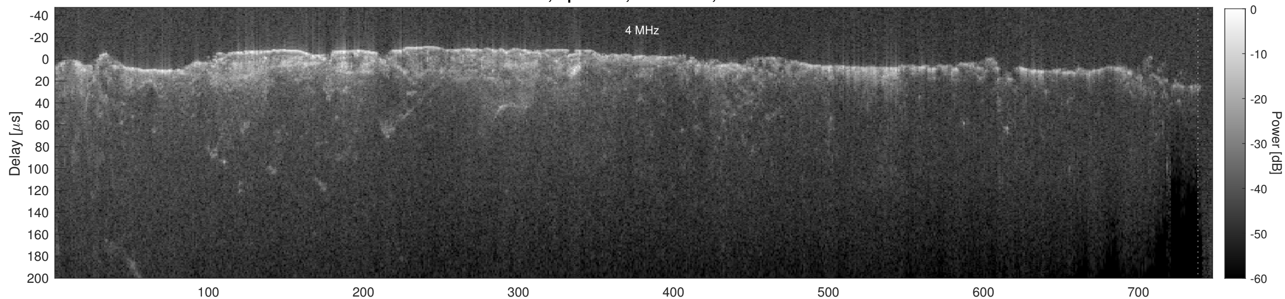
Orbit 6503, Cluttergram
