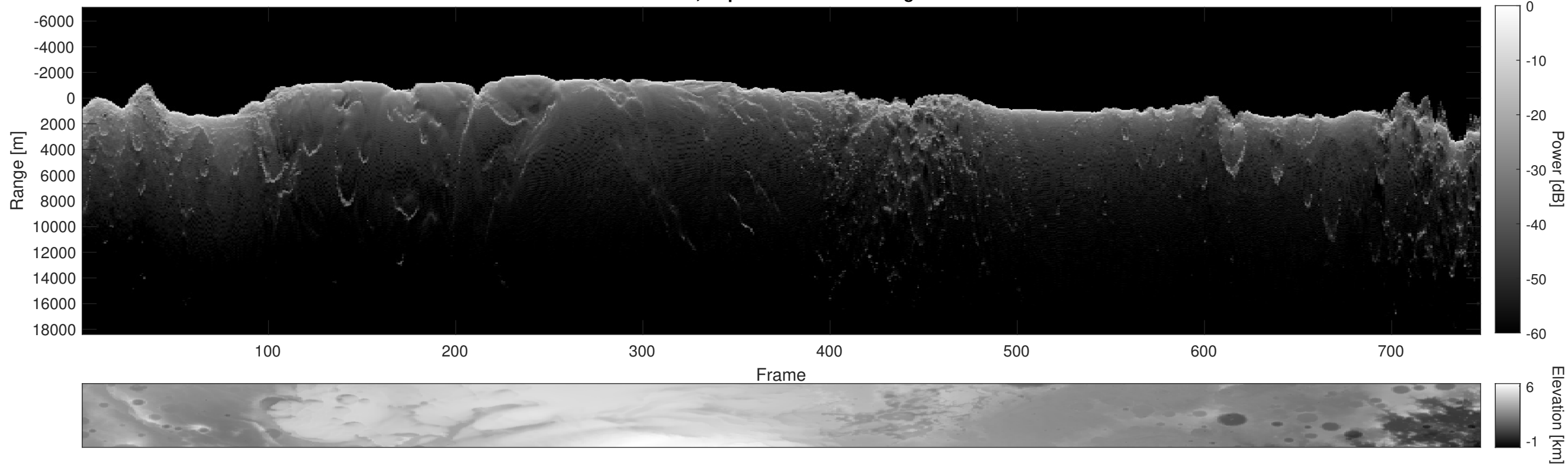
Orbit 6503, Depth-Corrected Cluttergram
