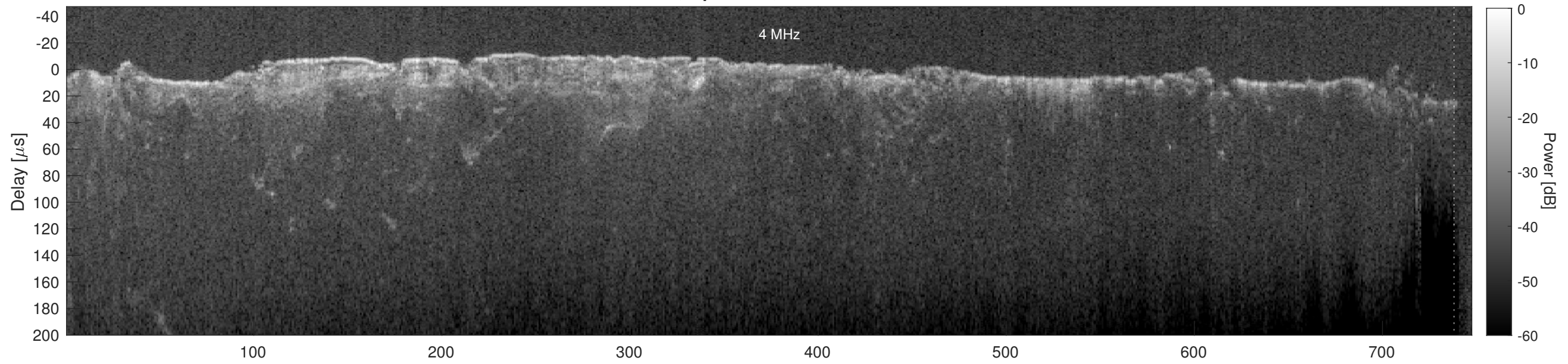
Orbit 6503, Cluttergram
