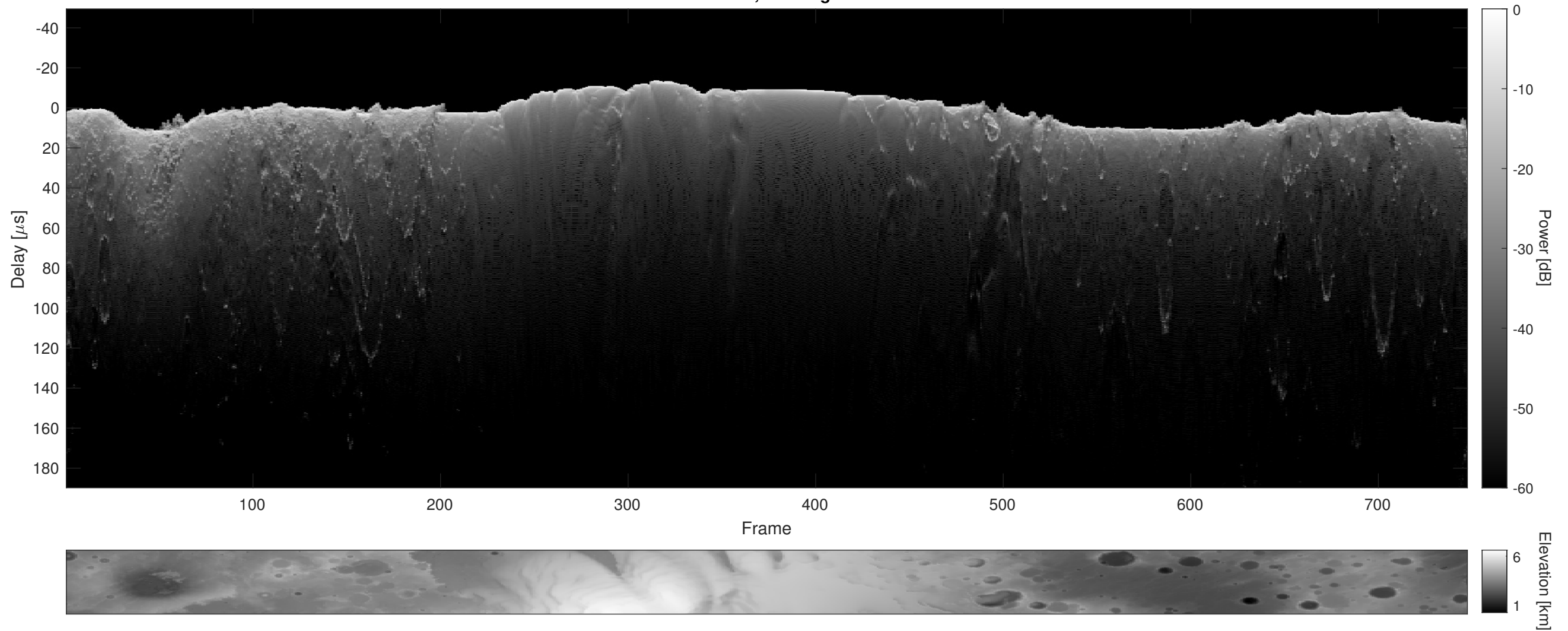
Orbit 6504, Cluttergram
