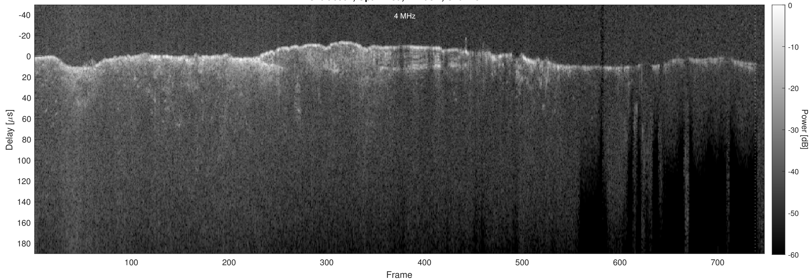
Orbit 6504, Optimized, Window, Channel 2
