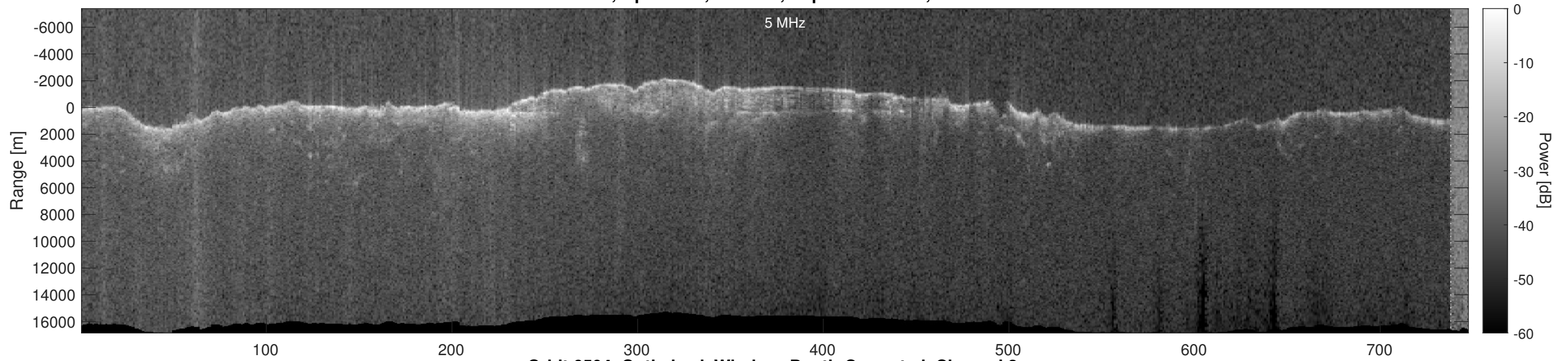
Orbit 6504, Optimized, Window, Depth-Corrected, Channel 2
