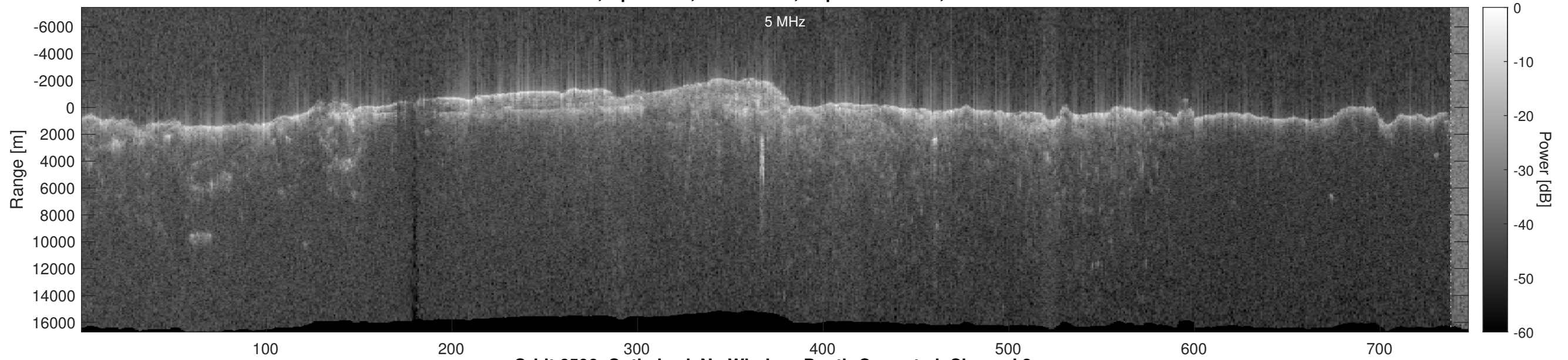
Orbit 6506, Optimized, No Window, Depth-Corrected, Channel 2
