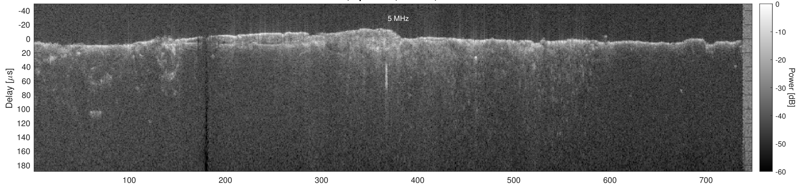
Orbit 6506, Optimized, Window, Channel 2
