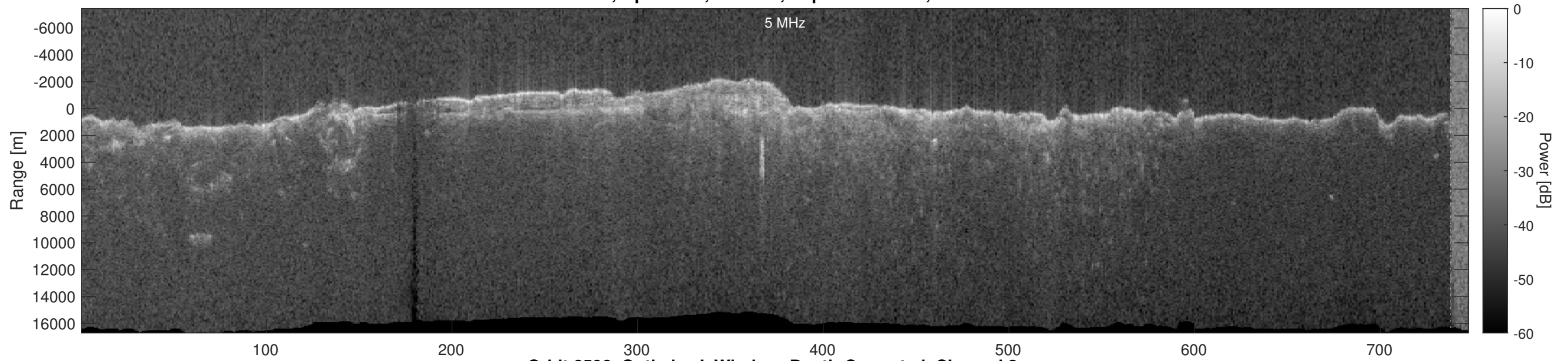
Orbit 6506, Optimized, Window, Depth-Corrected, Channel 2
