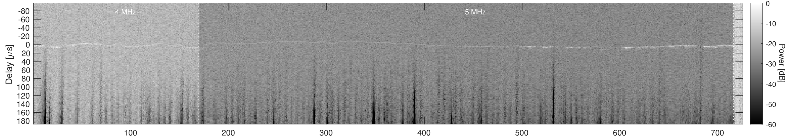
Orbit 6507, Cluttergram
