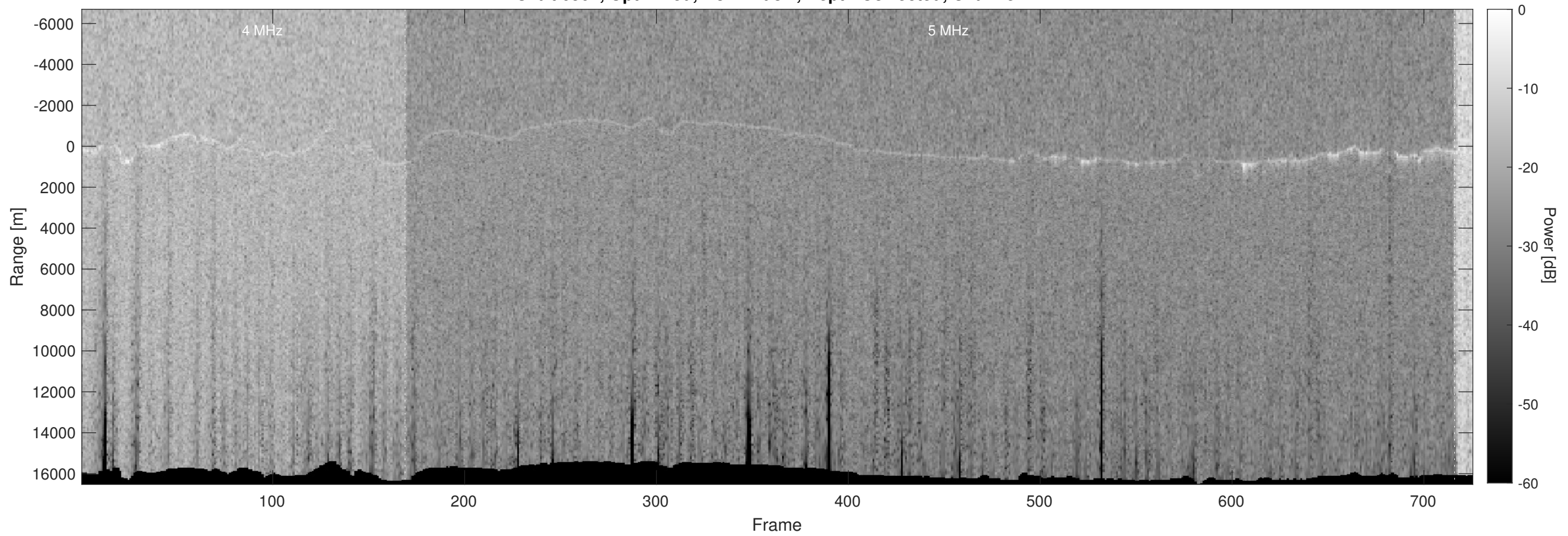
Orbit 6507, Optimized, No Window, Depth-Corrected, Channel 2
