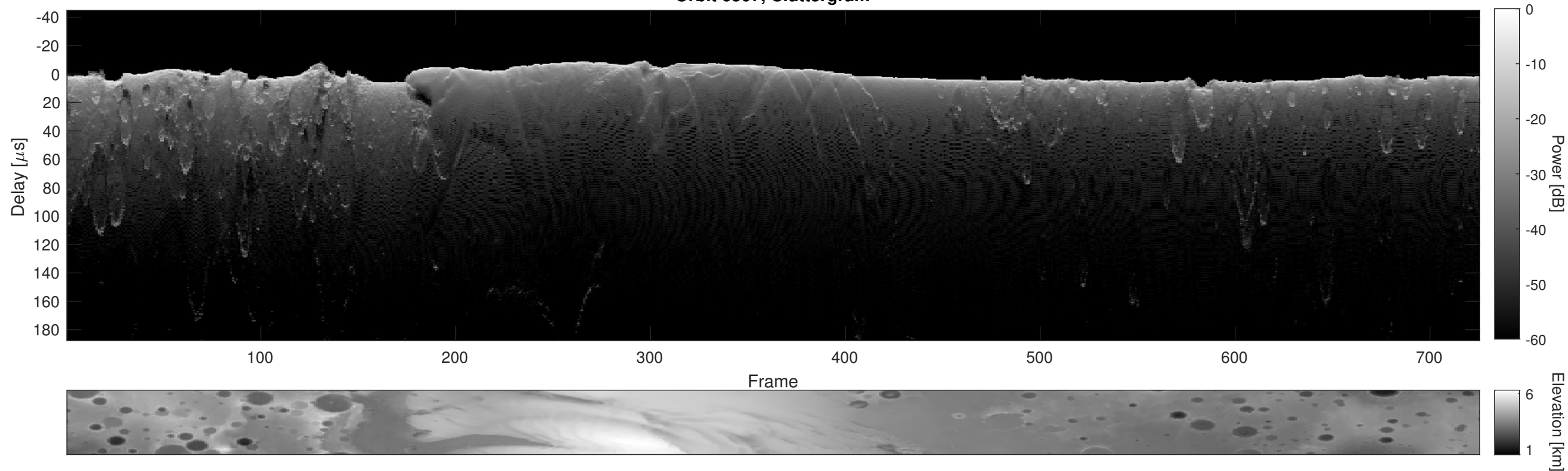
Orbit 6507, Cluttergram
