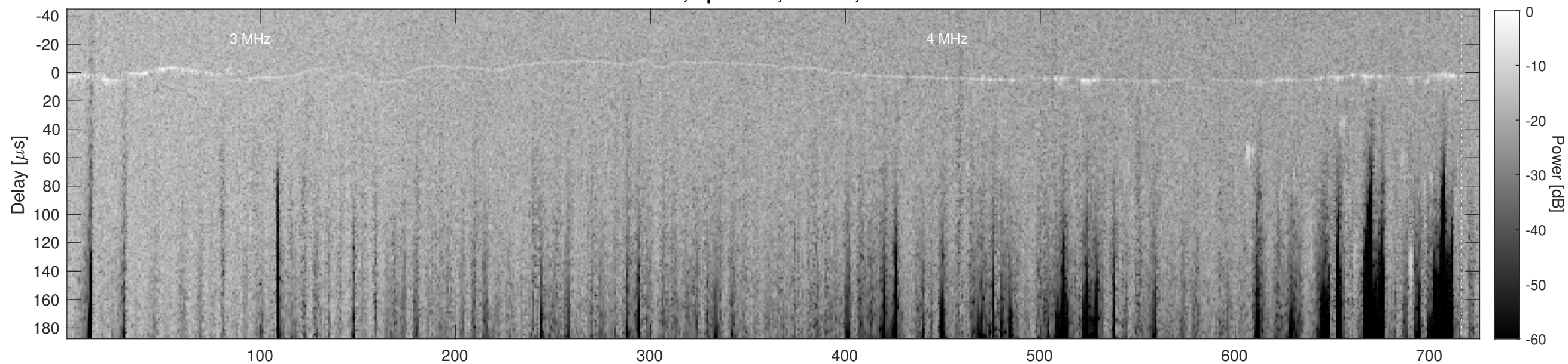
Orbit 6507, Cluttergram
