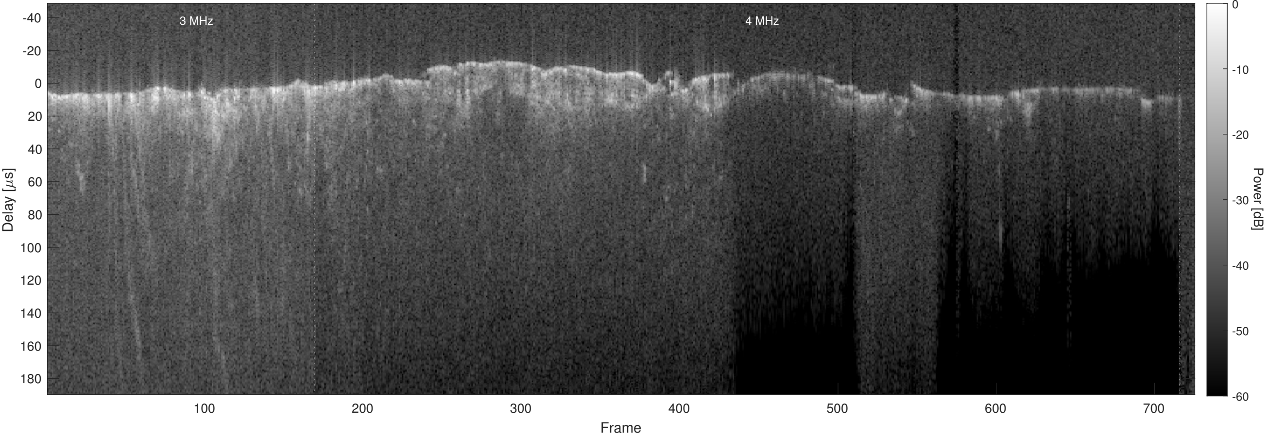
Orbit 6508, Optimized, No Window, Channel 2
