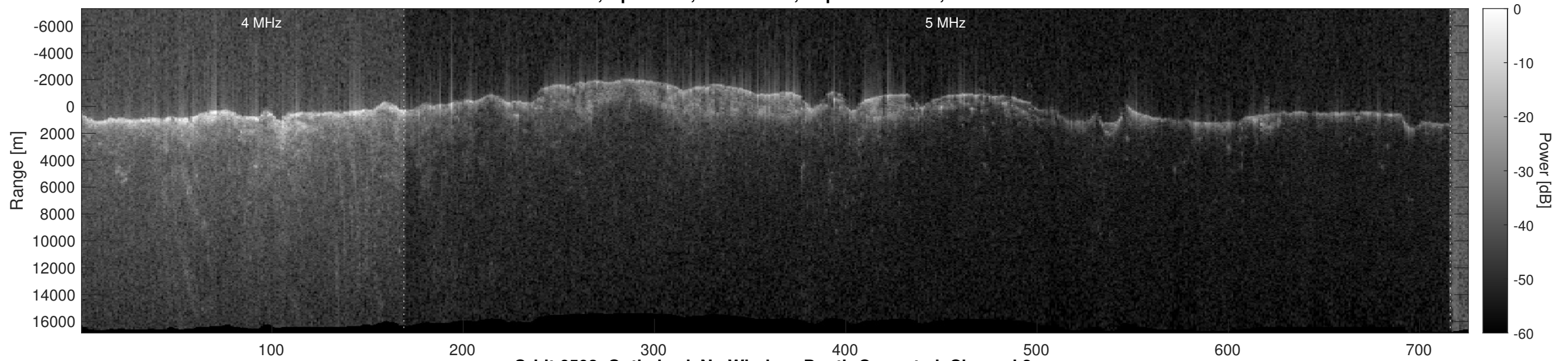
Orbit 6508, Optimized, No Window, Depth-Corrected, Channel 2
