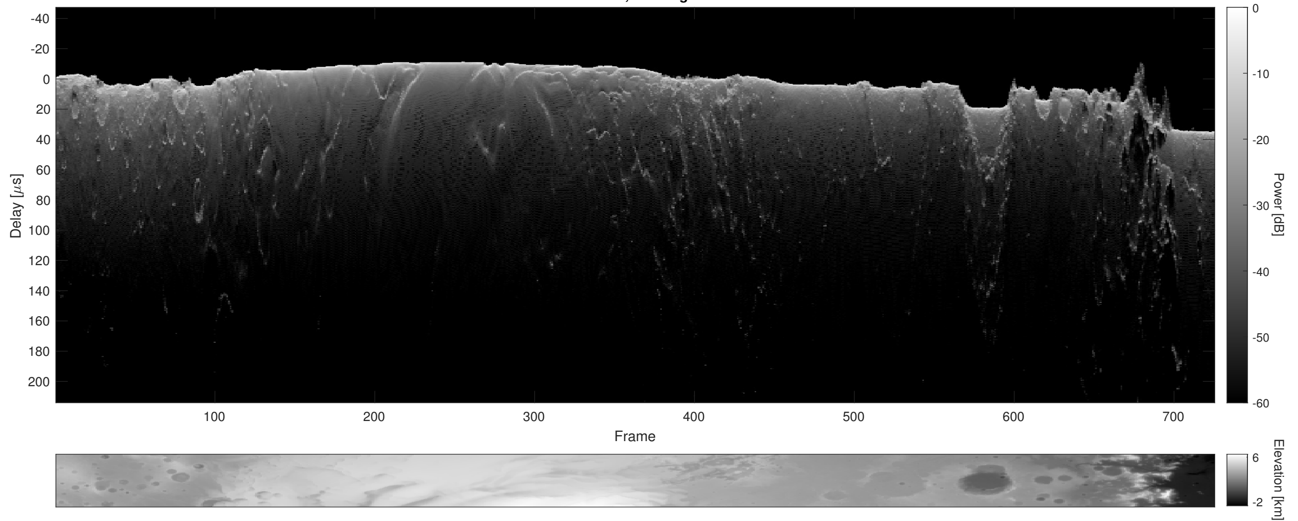
Orbit 6510, Cluttergram
