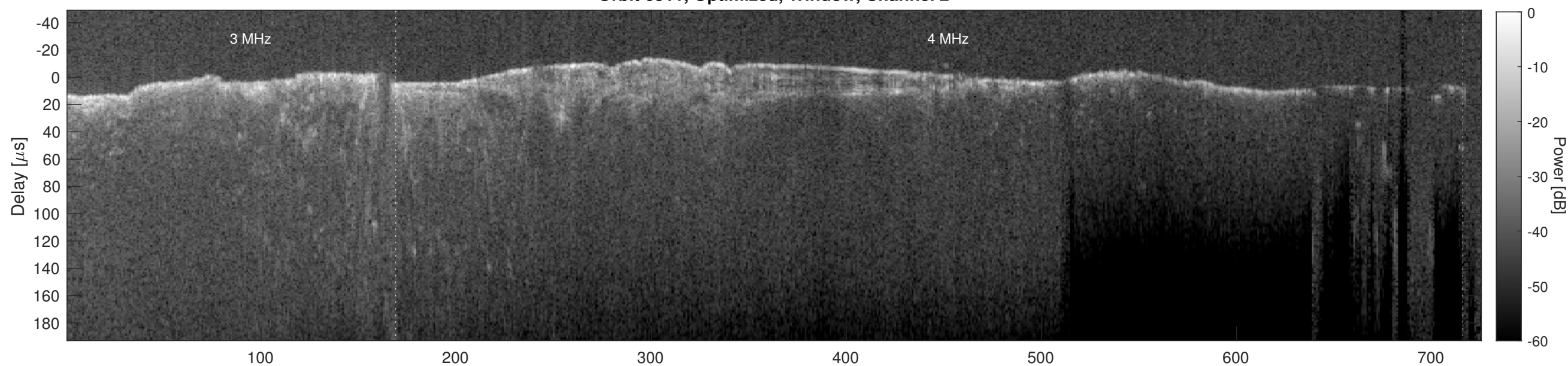
Orbit 6511, Cluttergram
