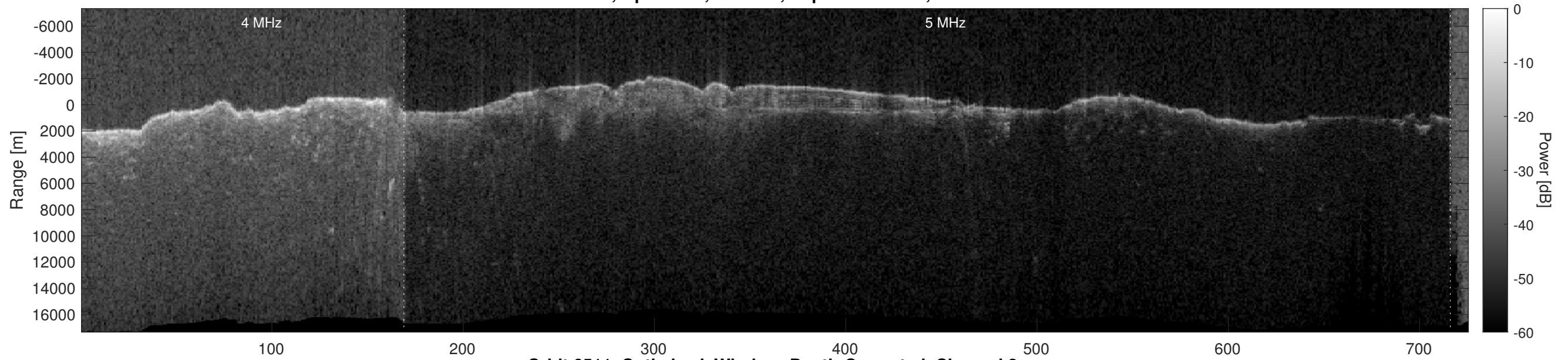
Orbit 6511, Optimized, Window, Depth-Corrected, Channel 2
