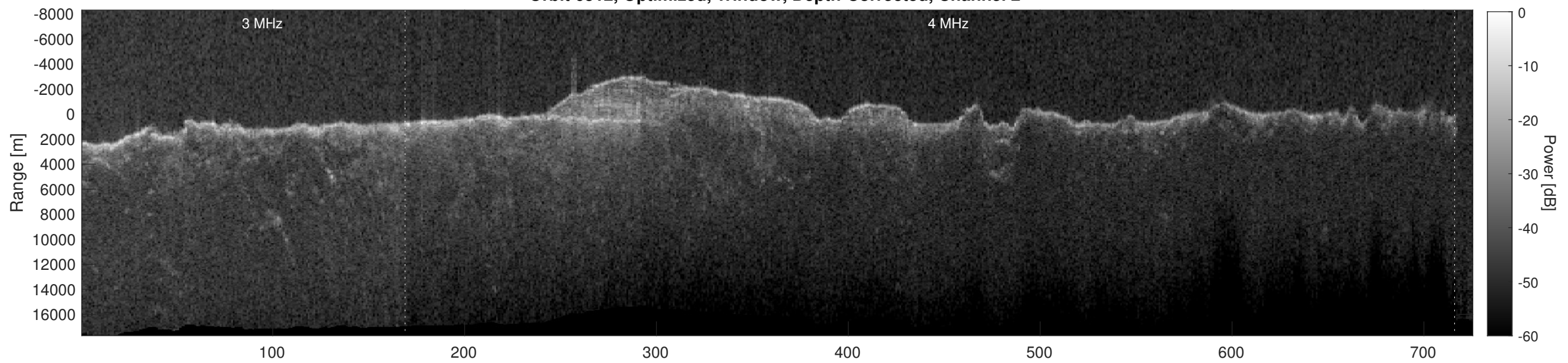
Orbit 6512, Depth-Corrected Cluttergram
