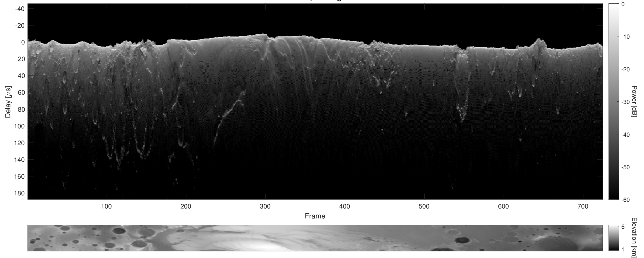
Orbit 6514, Cluttergram
