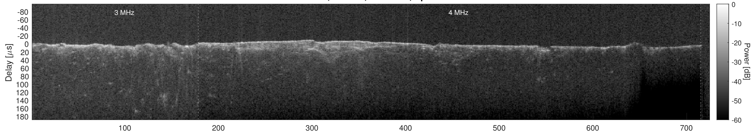
Orbit 6514, Cluttergram
