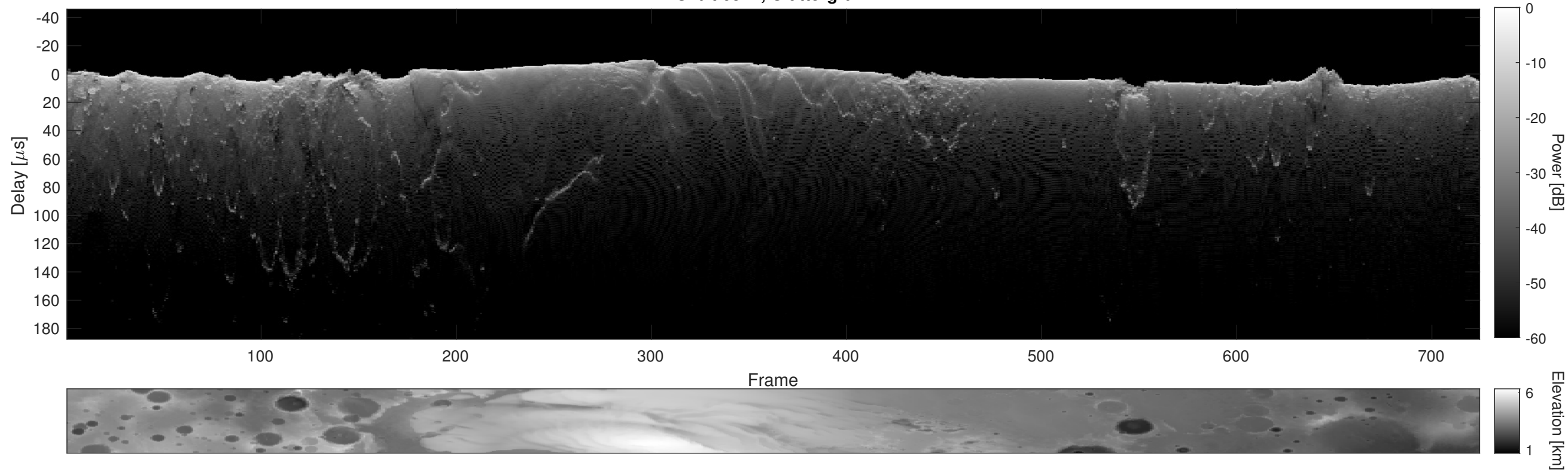
Orbit 6514, Cluttergram
