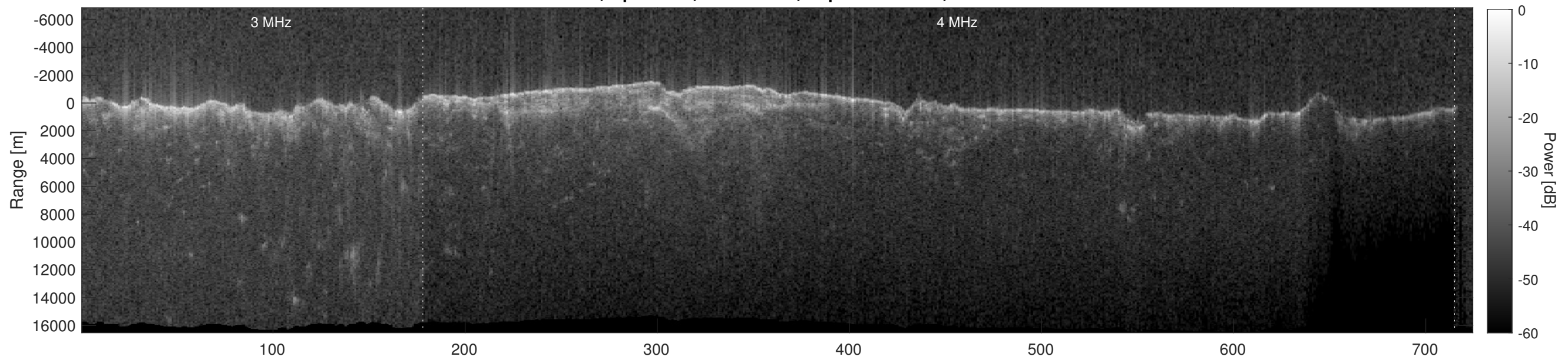
Orbit 6514, Depth-Corrected Cluttergram
