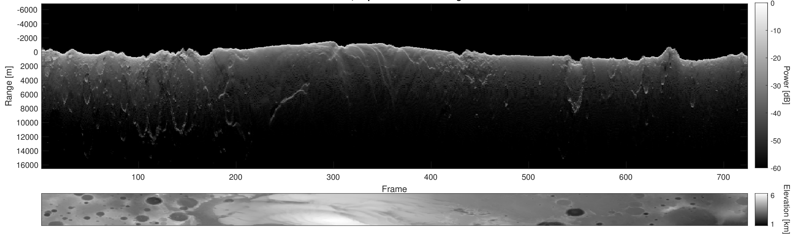
Orbit 6514, Depth-Corrected Cluttergram
