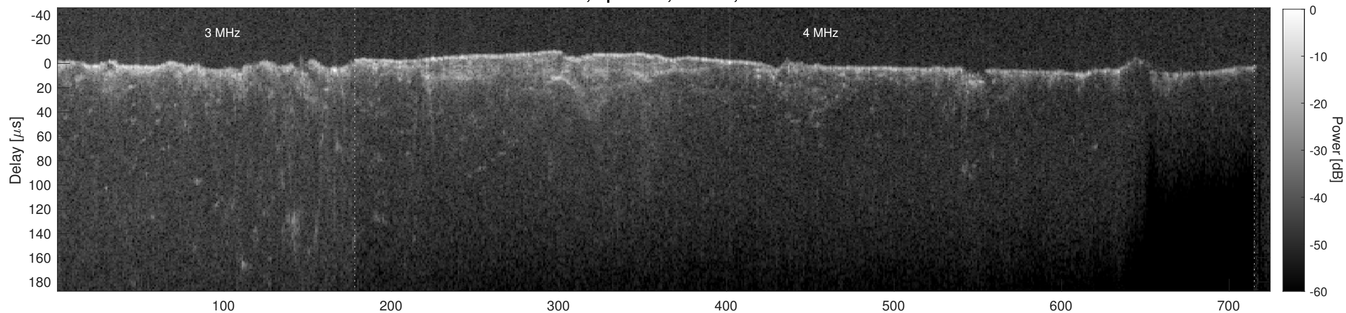
Orbit 6514, Cluttergram
