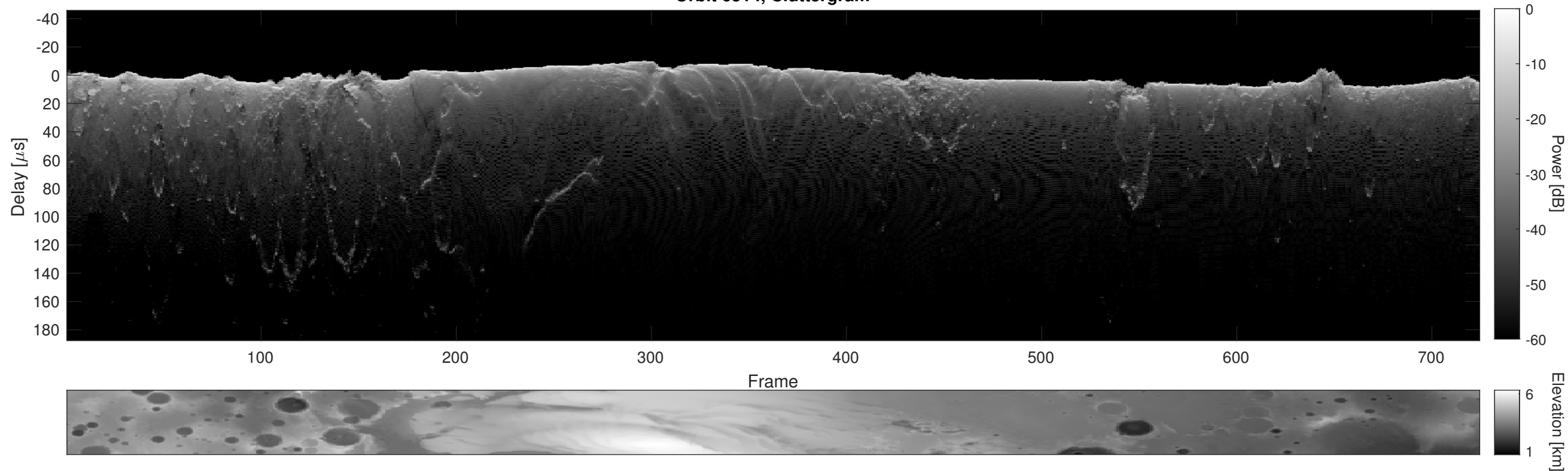
Orbit 6514, Cluttergram
