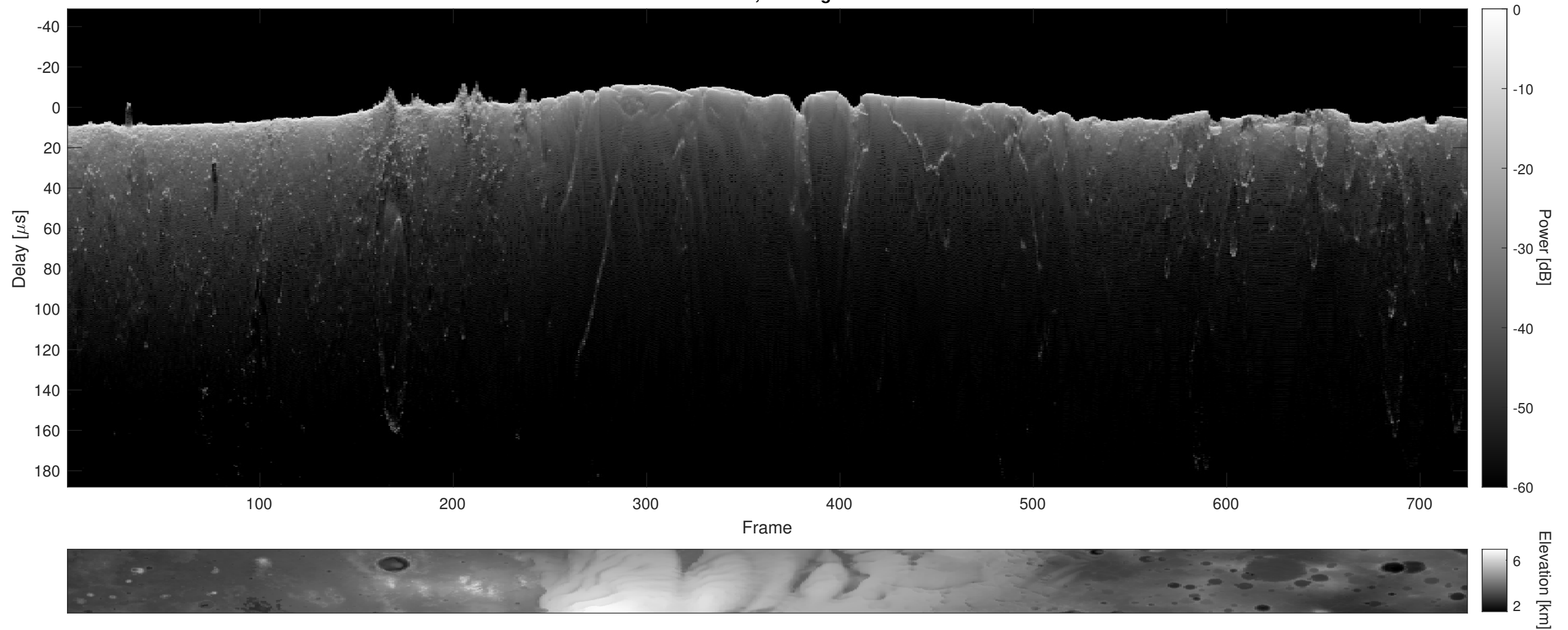
Orbit 6515, Cluttergram
