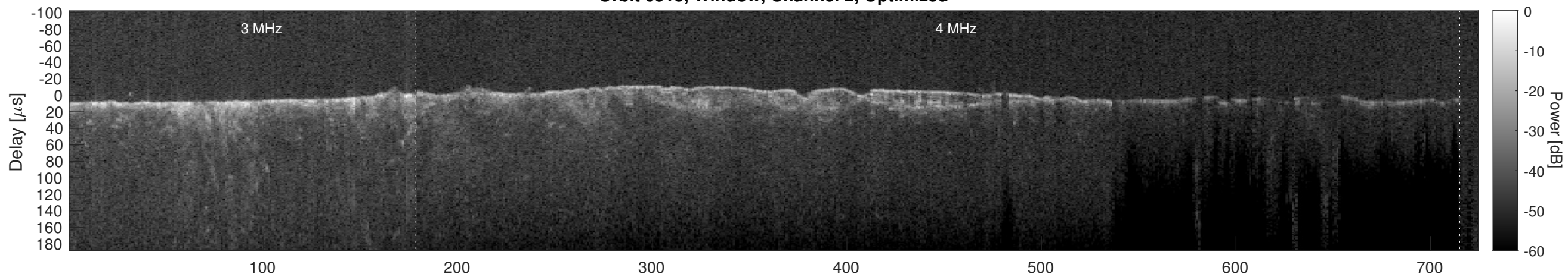
Orbit 6515, Cluttergram
