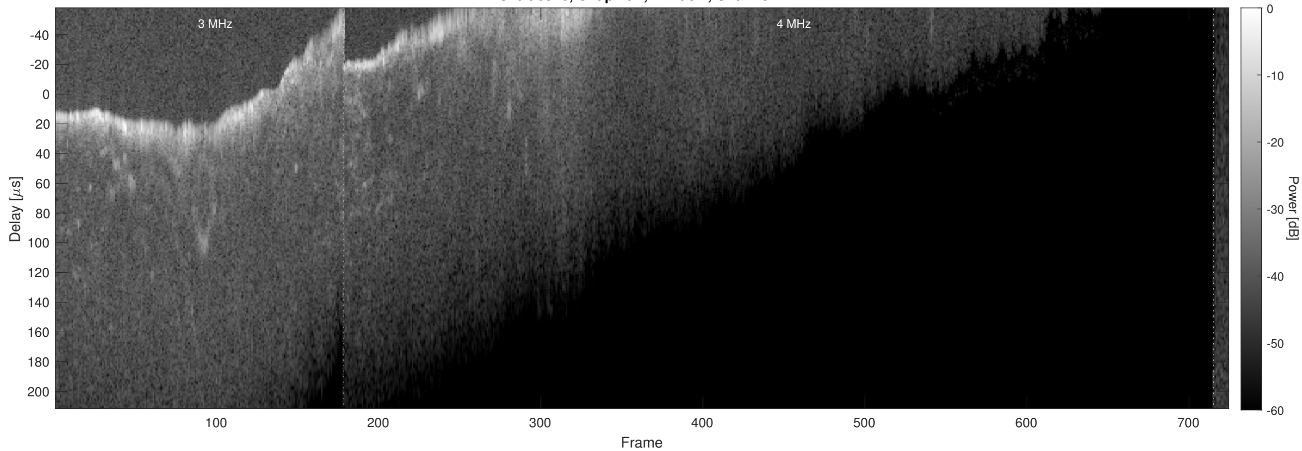
Orbit 6516, Chapman, Window, Channel 2
