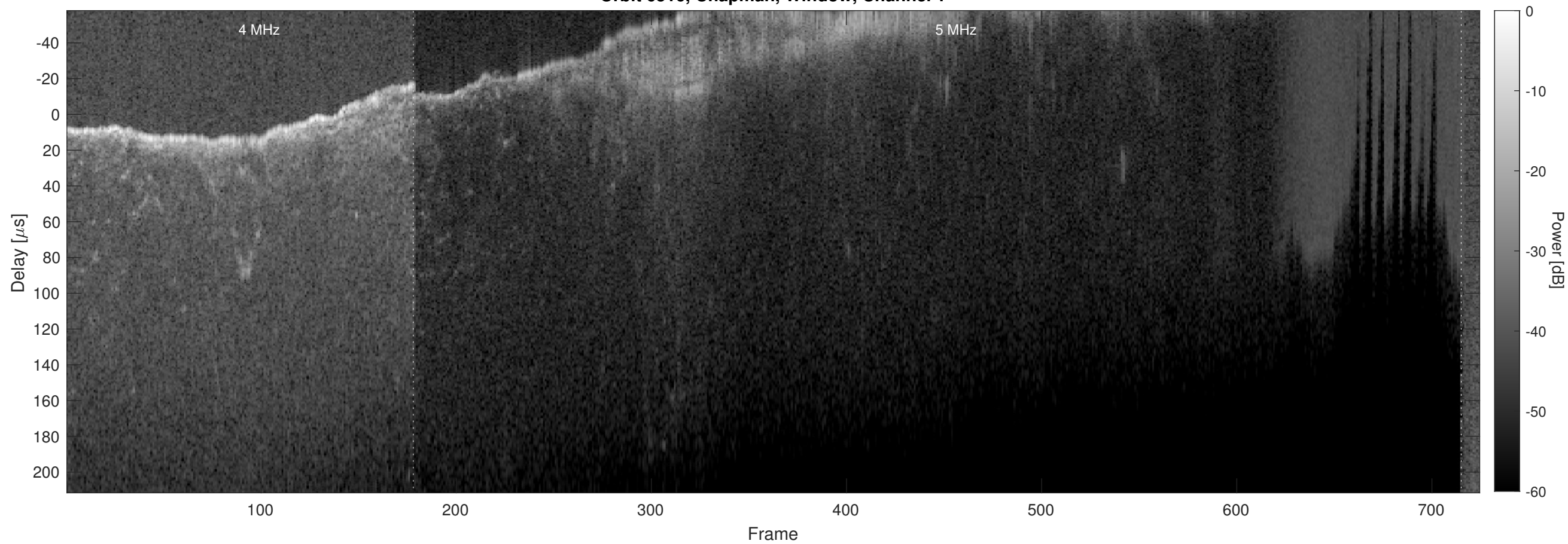
Orbit 6516, Chapman, Window, Channel 2
