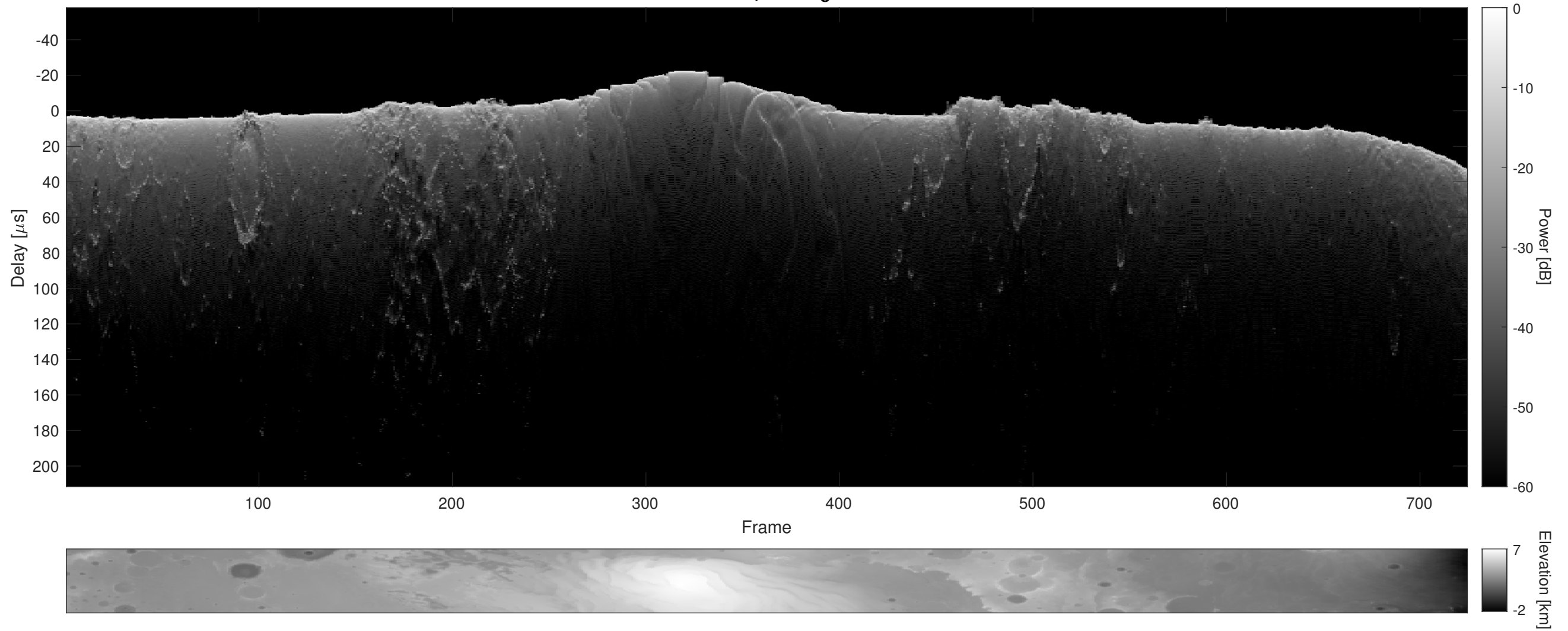
Orbit 6516, Cluttergram
