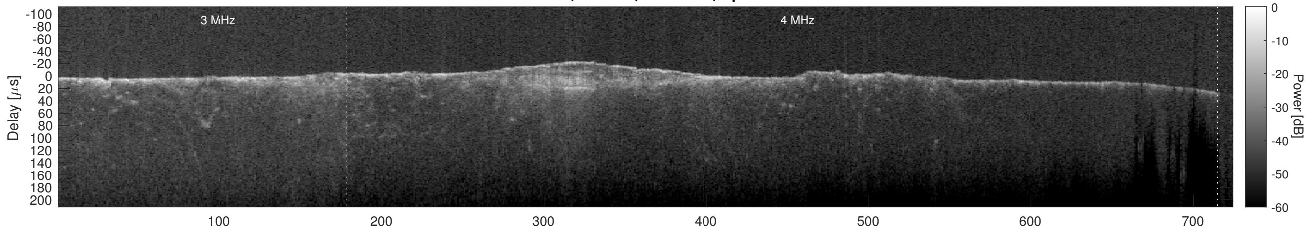
Orbit 6516, Cluttergram
