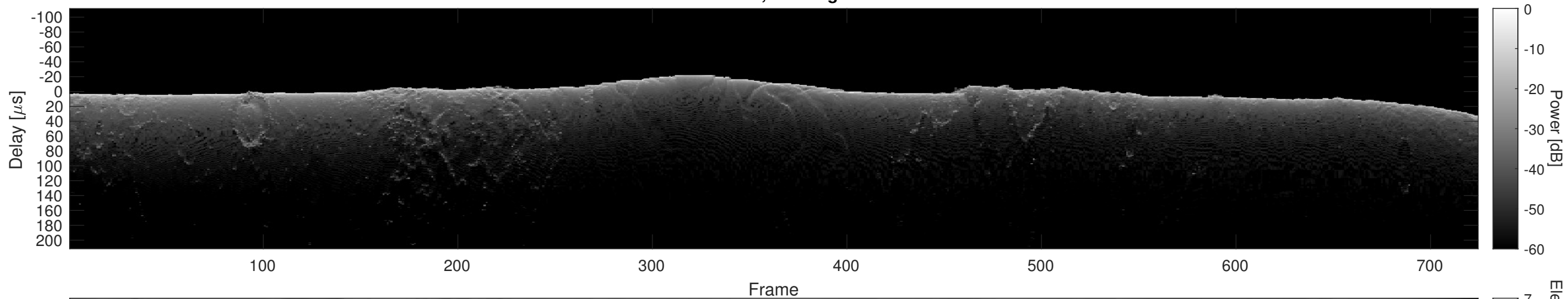
Orbit 6516, Cluttergram
