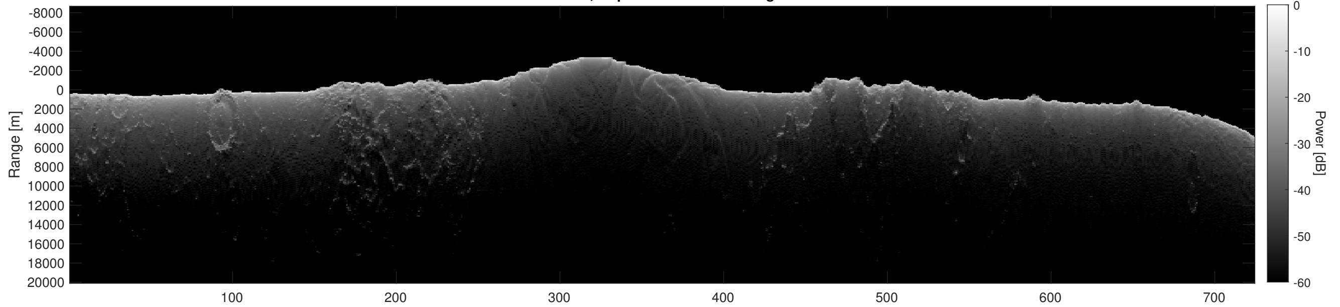
Orbit 6516, Depth-Corrected Cluttergram
