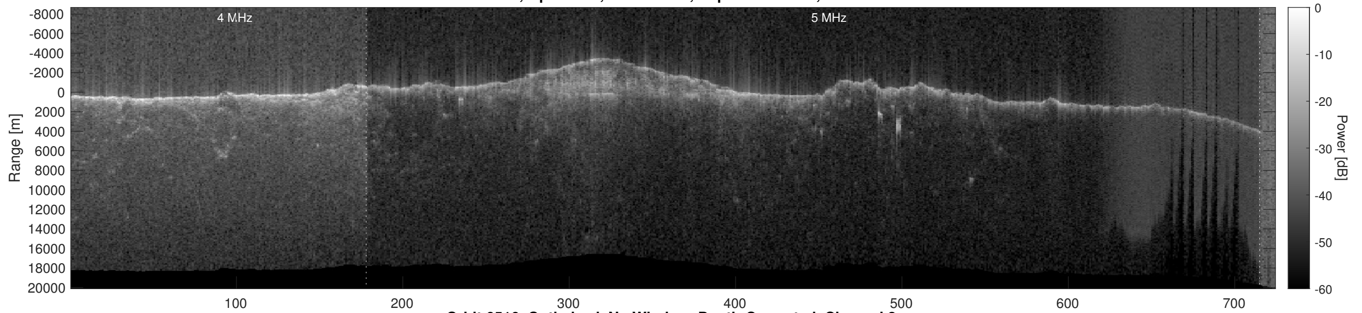
Orbit 6516, Optimized, No Window, Depth-Corrected, Channel 2
