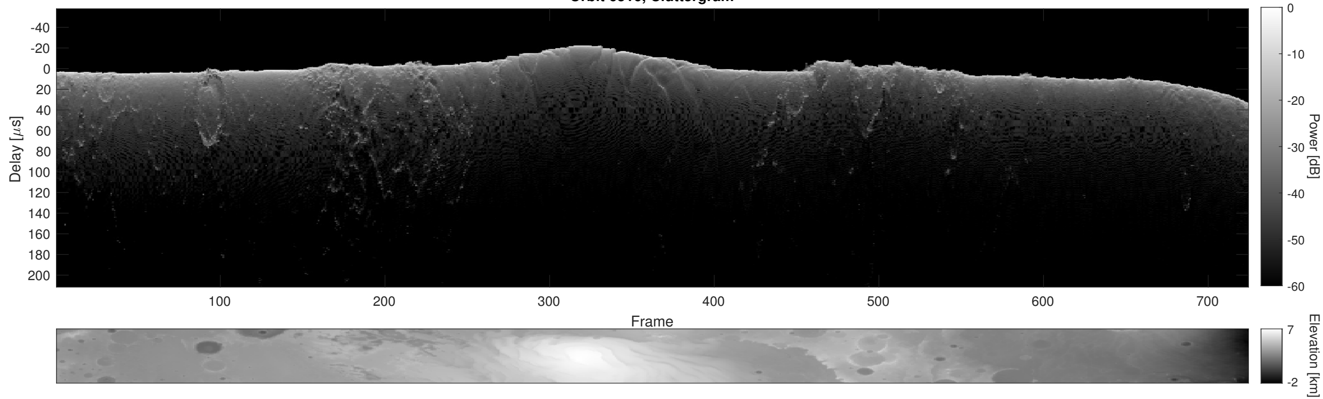
Orbit 6516, Cluttergram
