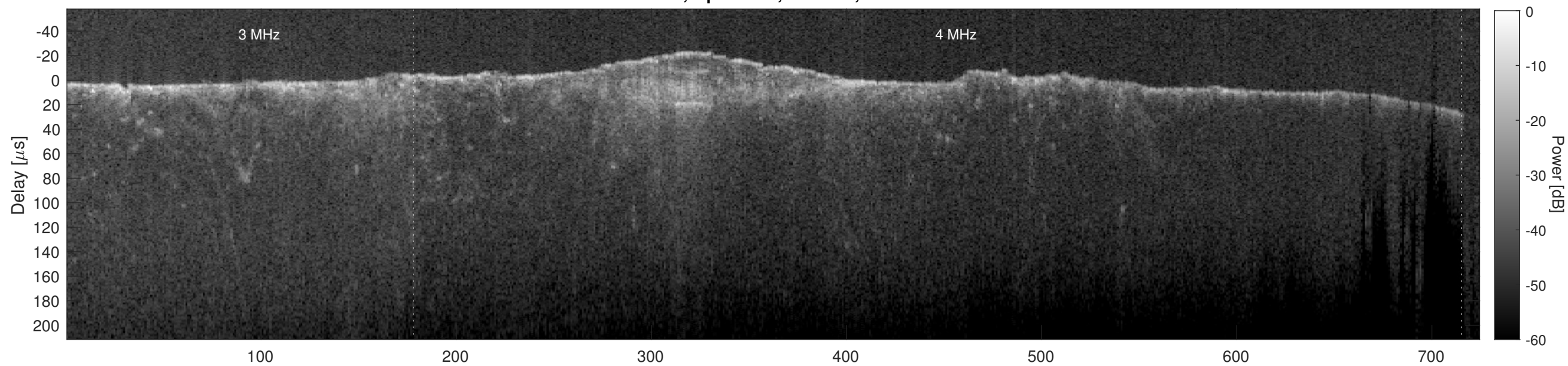
Orbit 6516, Cluttergram
