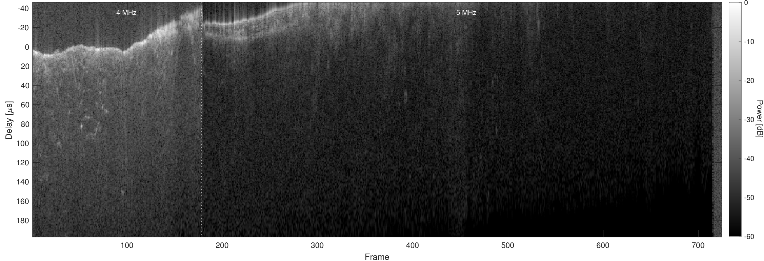
Orbit 6517, Chapman, No Window, Channel 2
