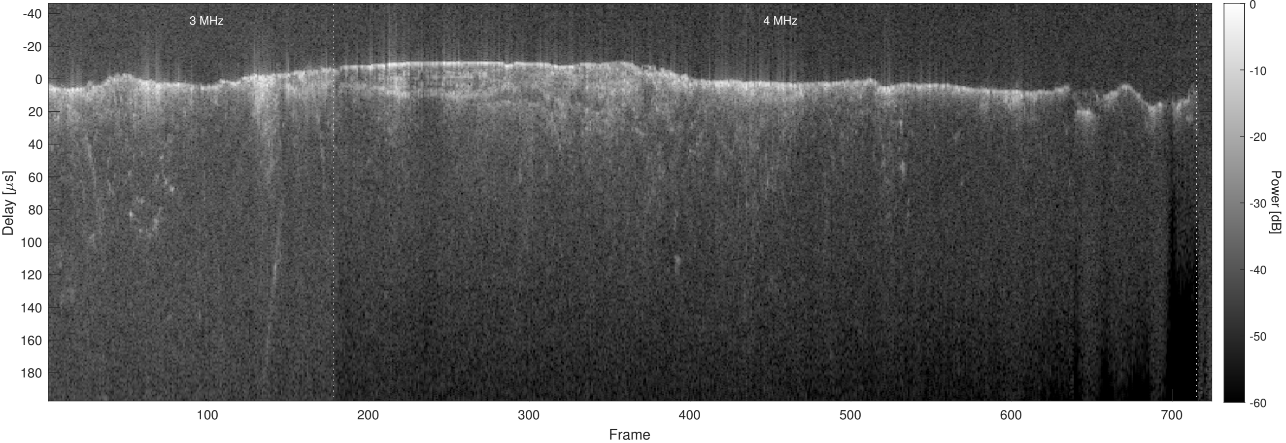
Orbit 6517, Optimized, No Window, Channel 2
