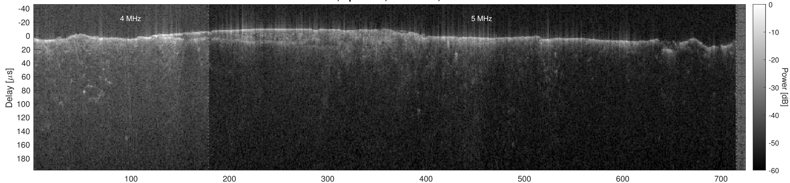
Orbit 6517, Optimized, No Window, Channel 2
