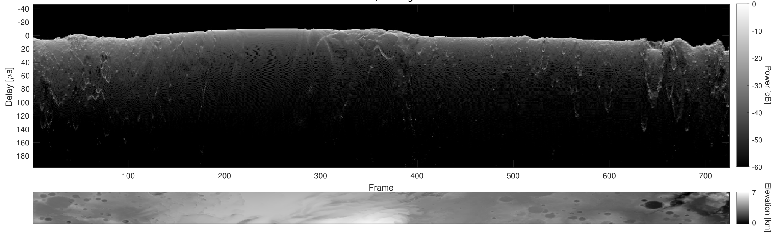
Orbit 6517, Cluttergram
