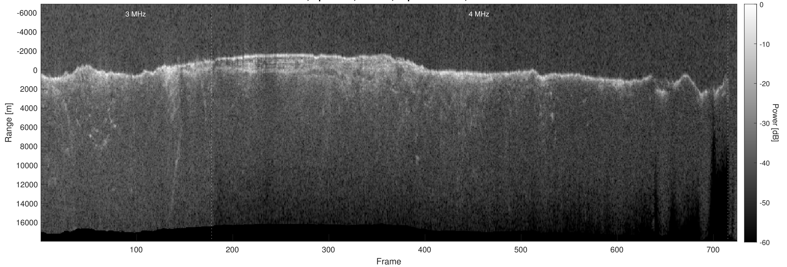
Orbit 6517, Optimized, Window, Depth-Corrected, Channel 2
