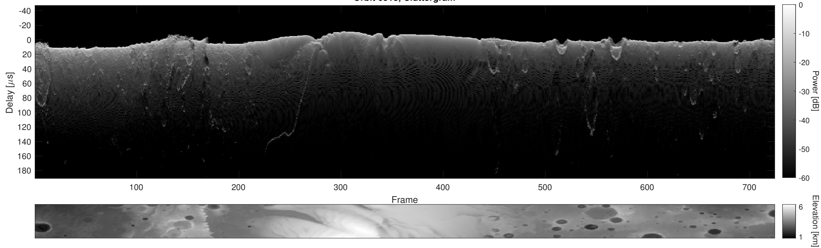
Orbit 6518, Cluttergram
