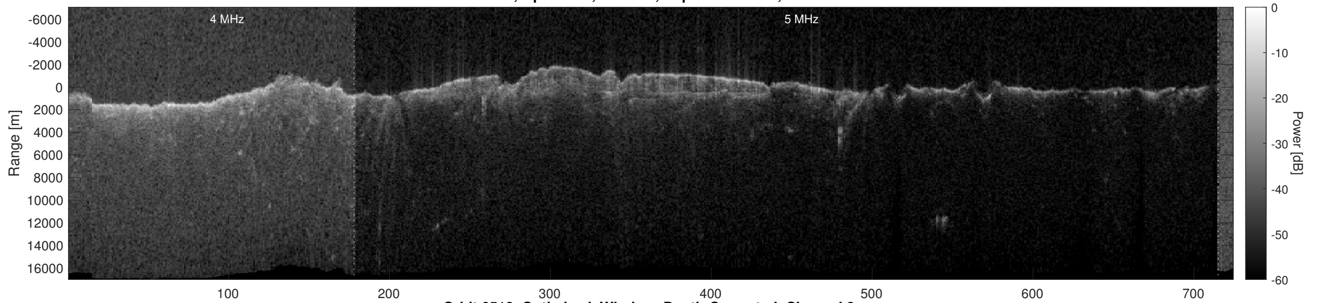
Orbit 6518, Optimized, Window, Depth-Corrected, Channel 2
