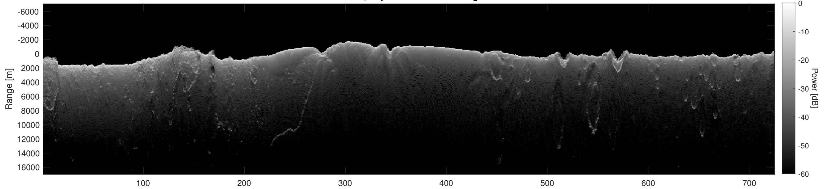
Orbit 6518, Depth-Corrected Cluttergram
