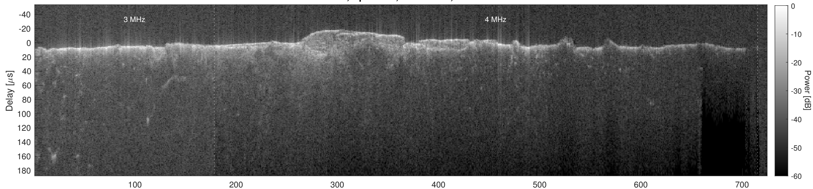
Orbit 6519, Cluttergram
