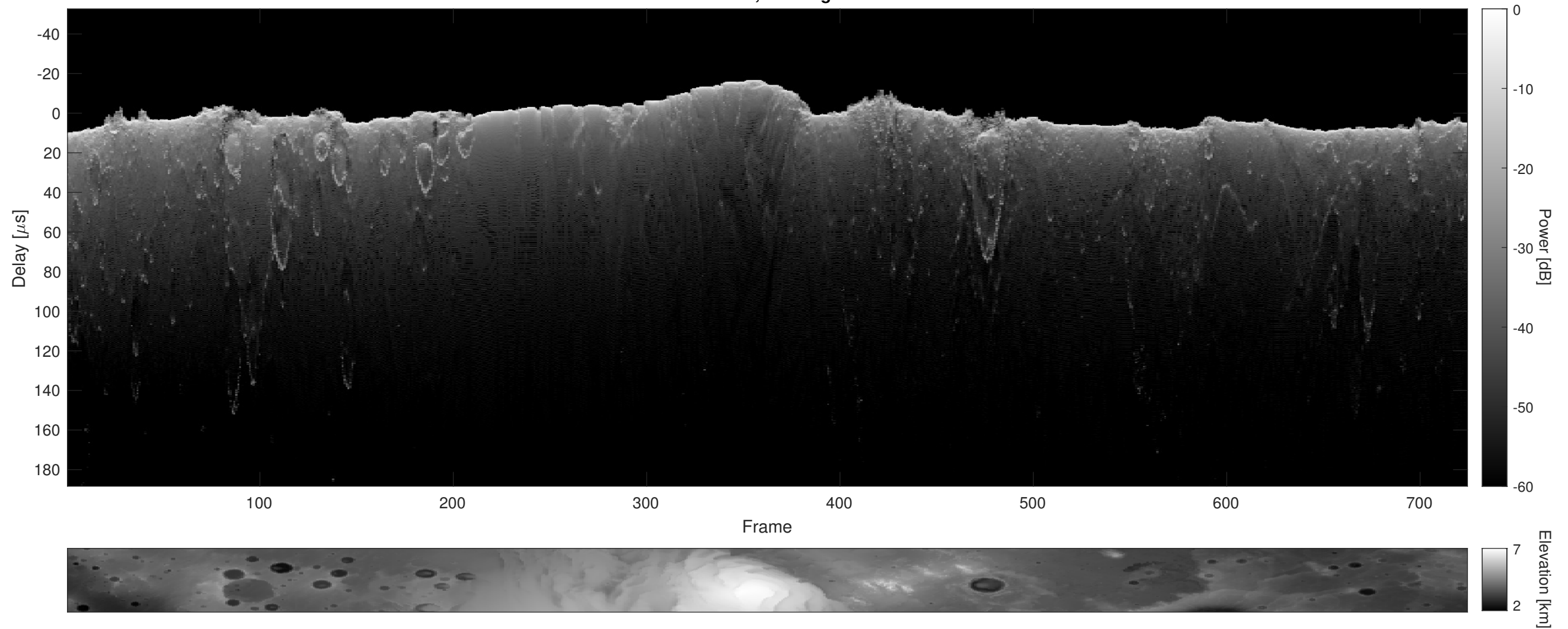
Orbit 6520, Cluttergram
