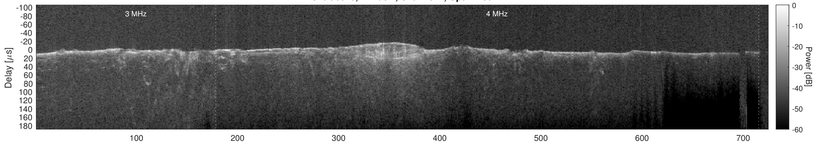
Orbit 6520, Cluttergram
