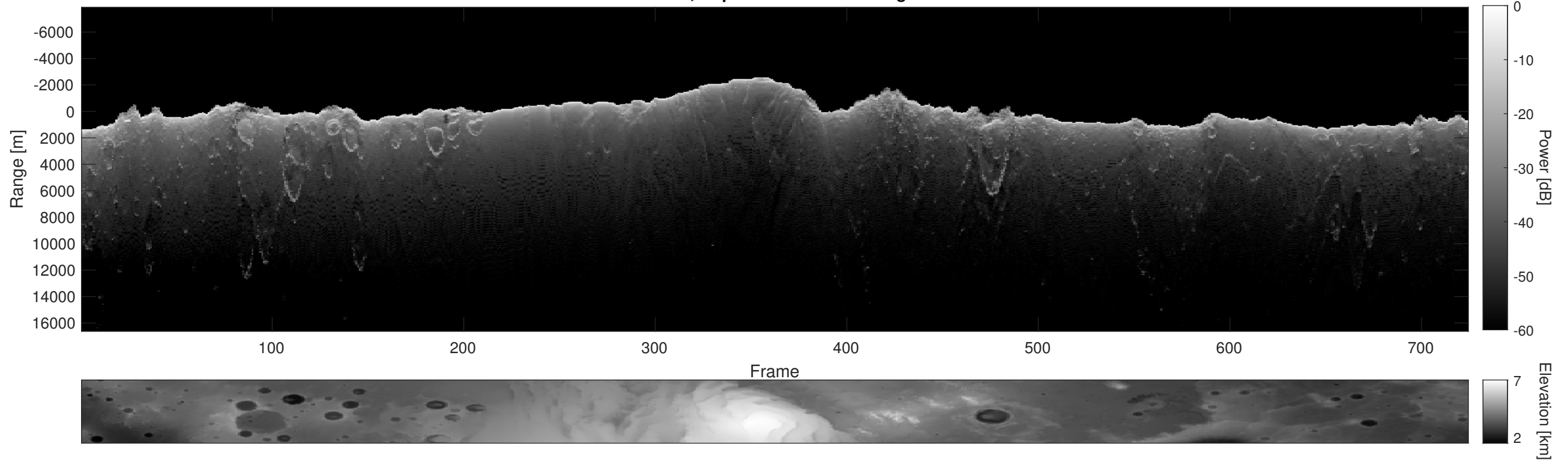
Orbit 6520, Depth-Corrected Cluttergram
