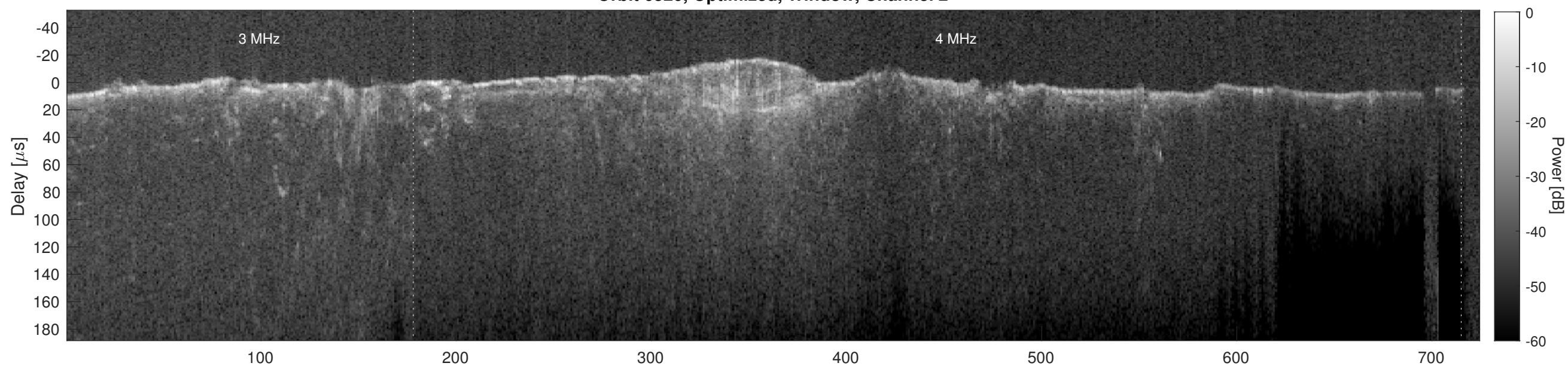
Orbit 6520, Cluttergram
