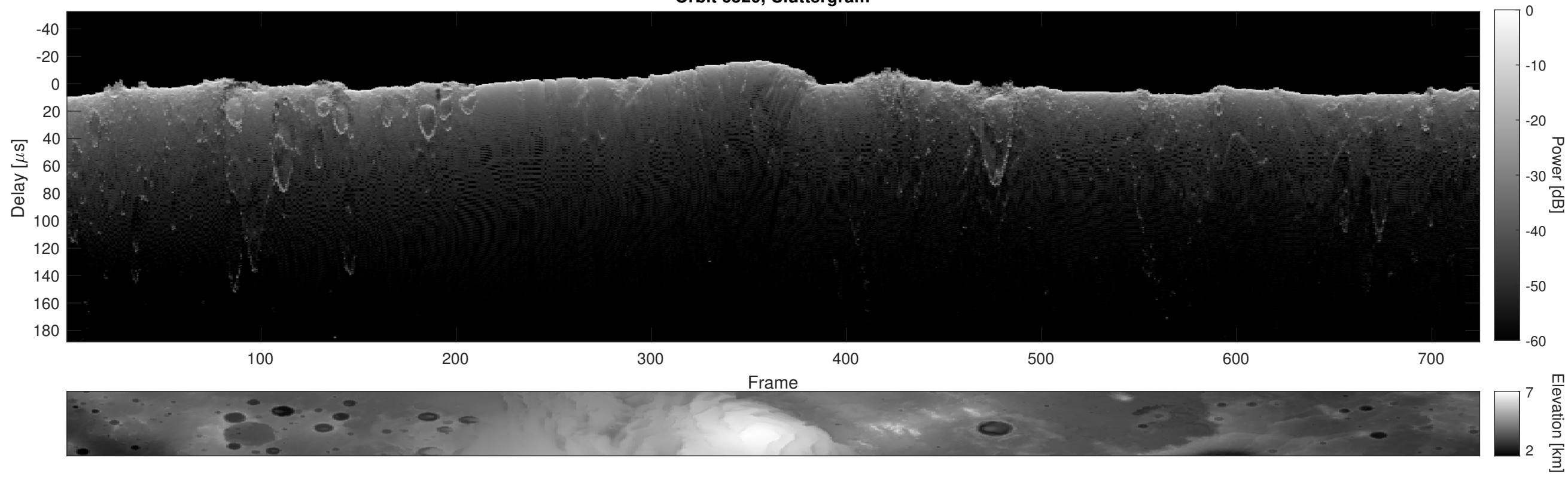
Orbit 6520, Cluttergram
