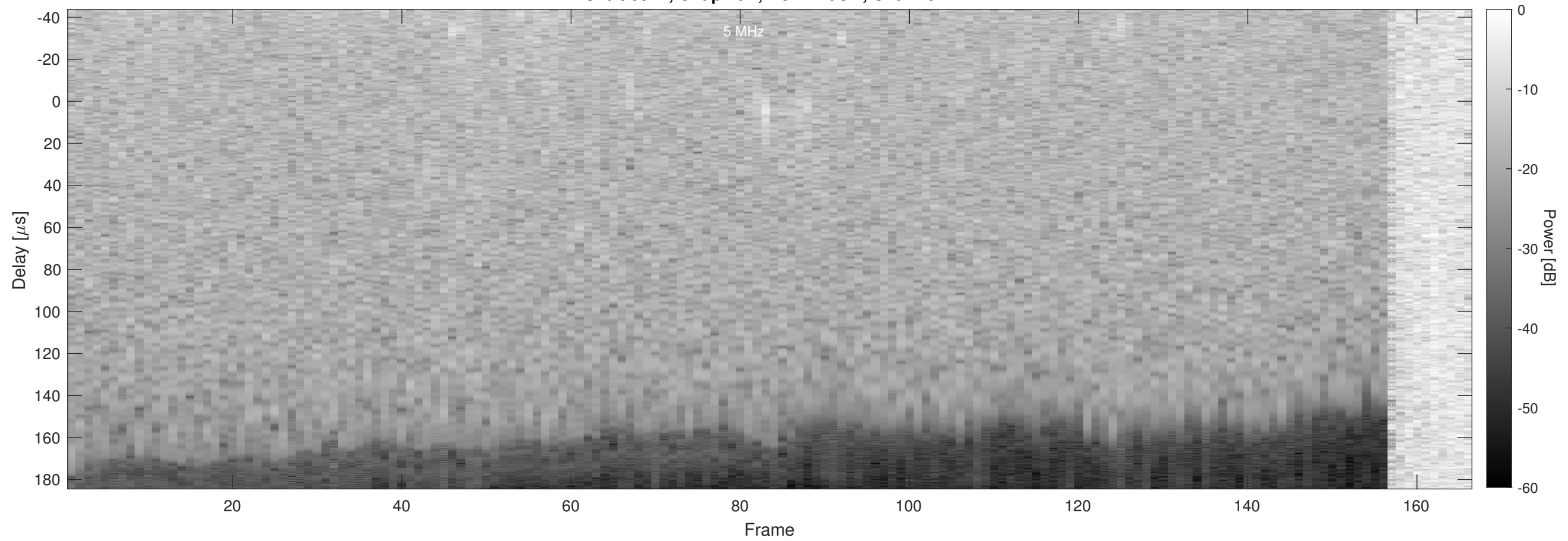
Orbit 6521, Chapman, No Window, Channel 2
