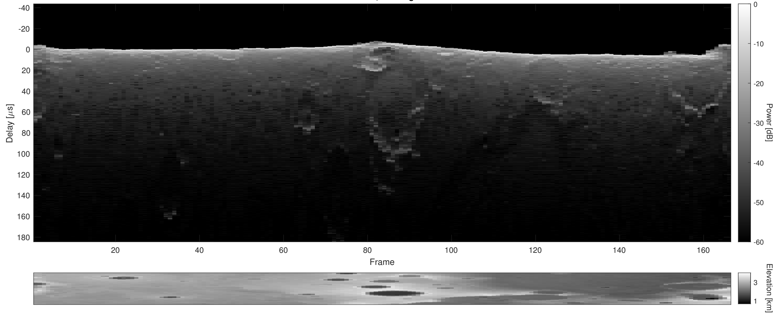
Orbit 6521, Cluttergram
