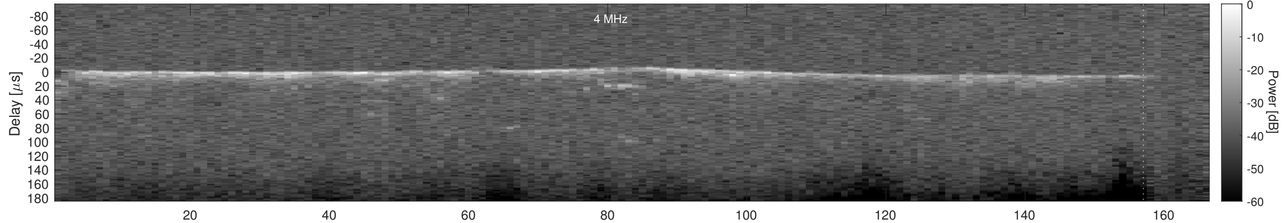
Orbit 6521, Cluttergram
