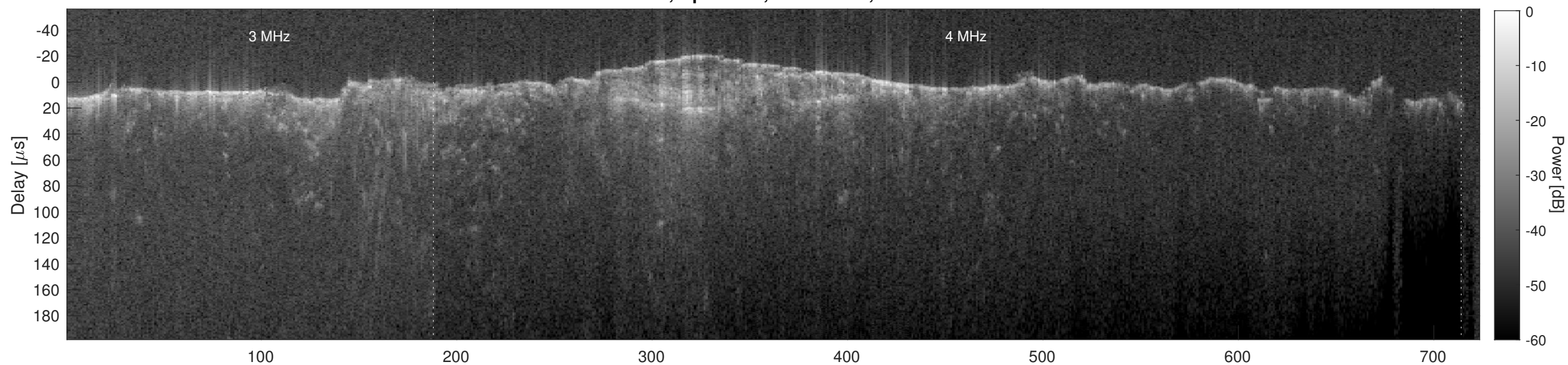
Orbit 6523, Cluttergram
