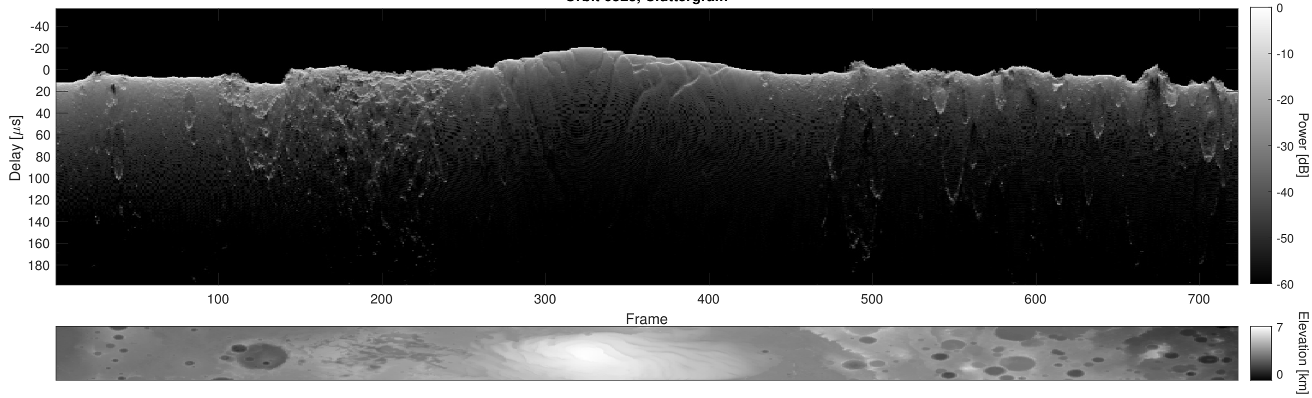
Orbit 6523, Cluttergram
